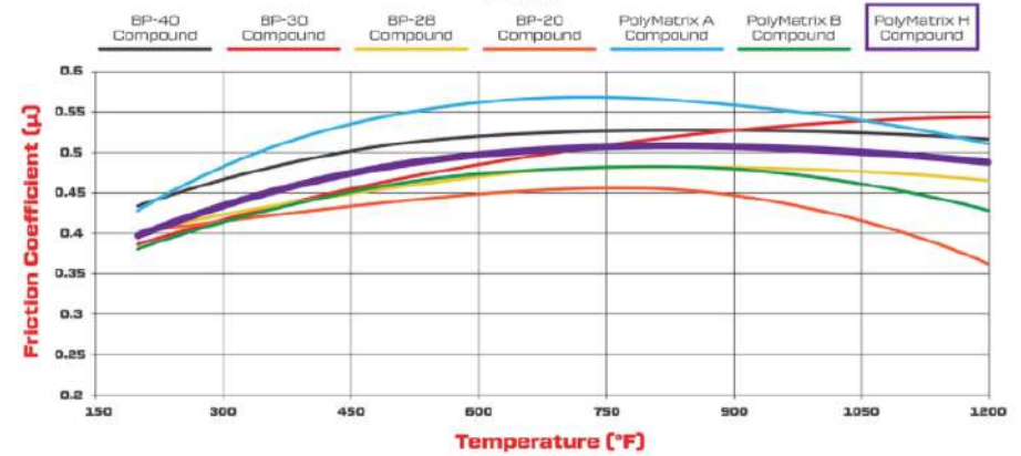
PolyMatrix H Friction Coefficient and Temperature Values
